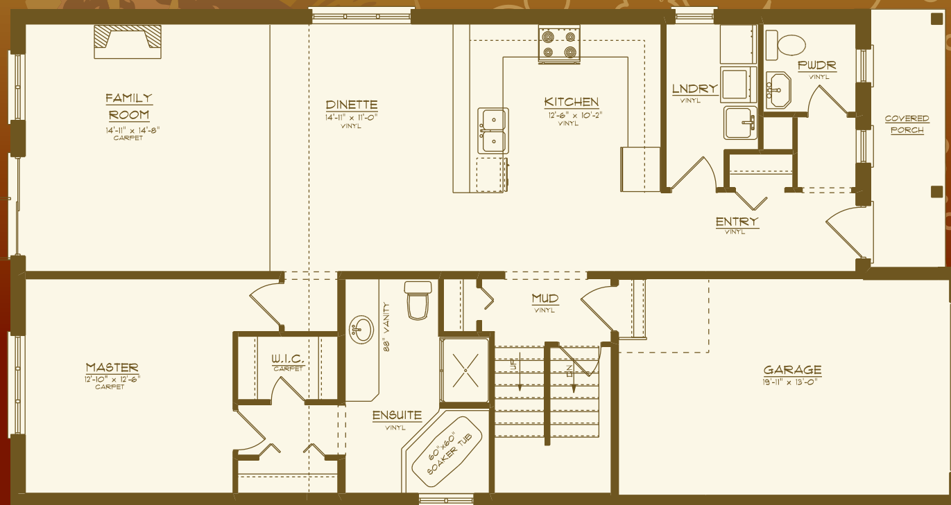
Main Floor 1,342 Sq. Ft.
